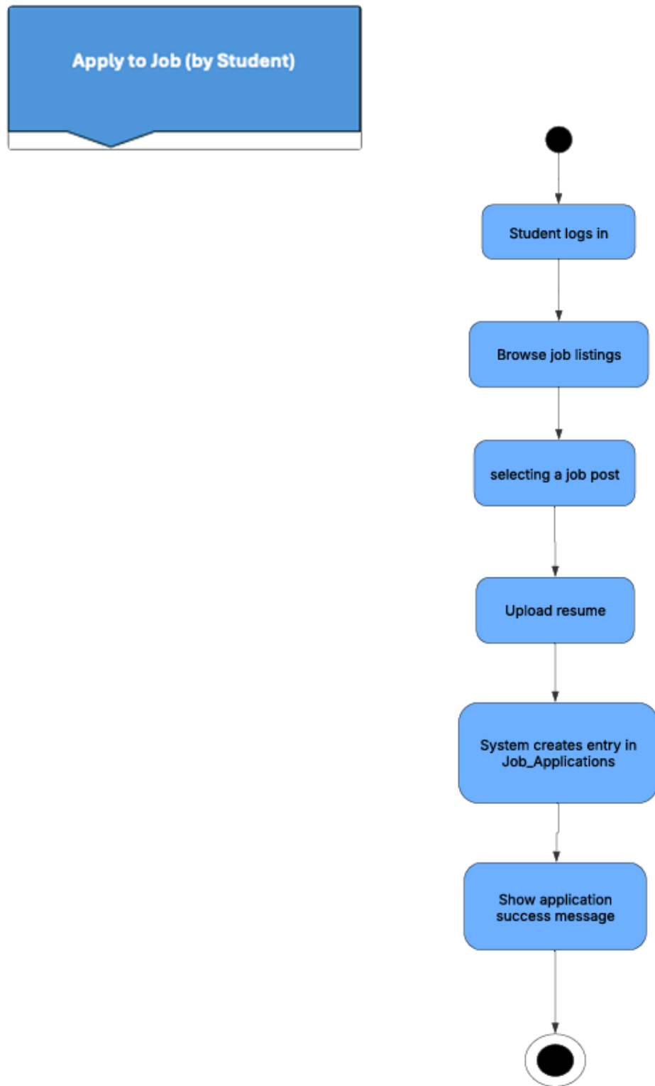
Figure 14. Activity Diagram (Apply to job)
