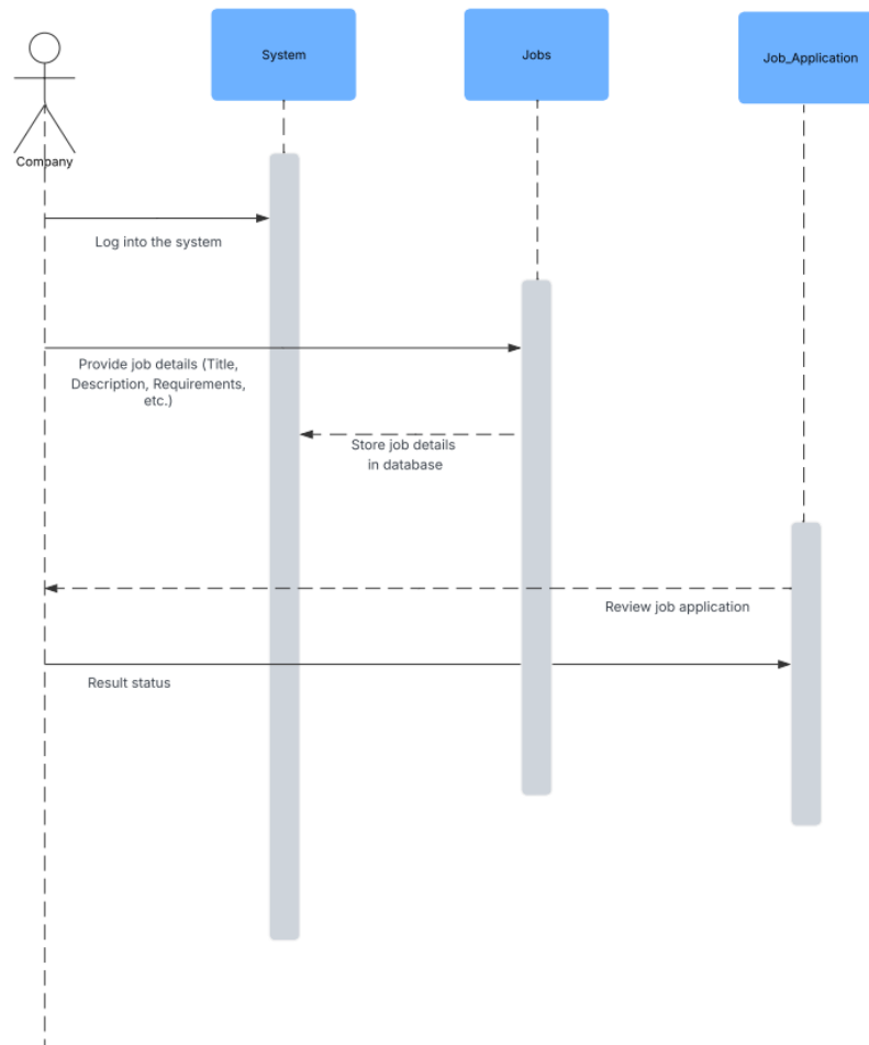
Figure 10. Sequence Diagram (Company)
