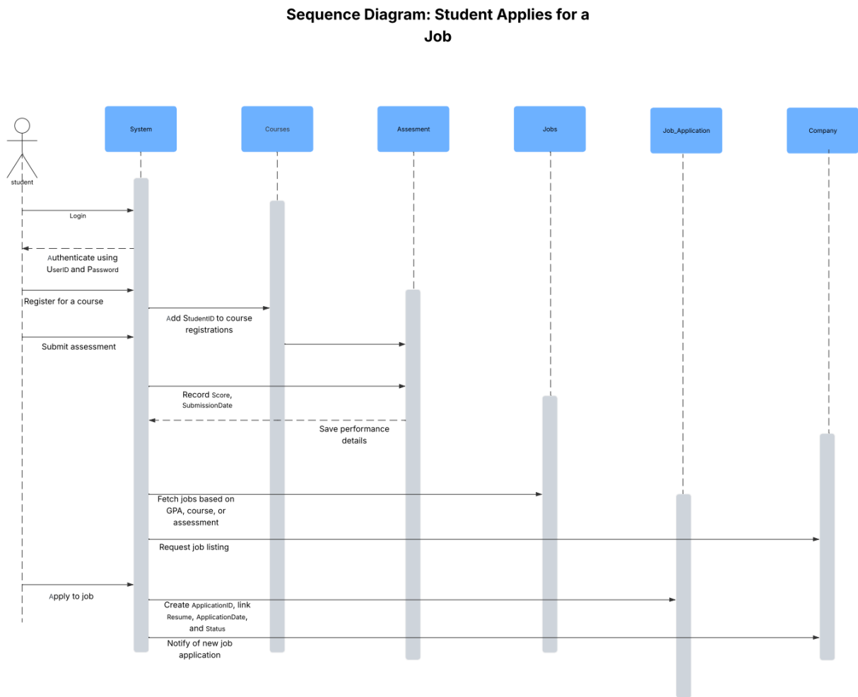
Figure 7. Sequence Diagram (Student)
